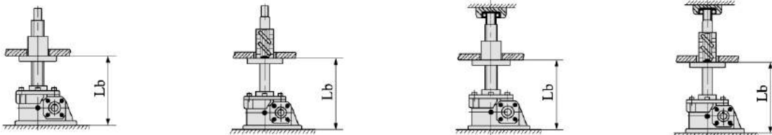
轴端自由 f_n=0.36 Movable shaft end f_n=0.36
